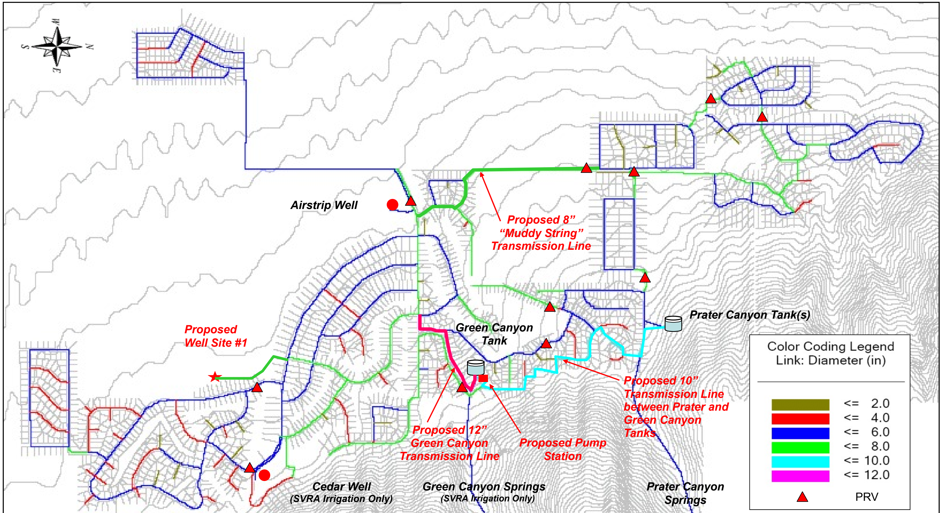
Figure 7.1 PROPOSED STAR VALLEY RANCH WATER SYSTEM Future Line Sizes
